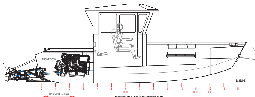
SECTION AT CENTERLINE
