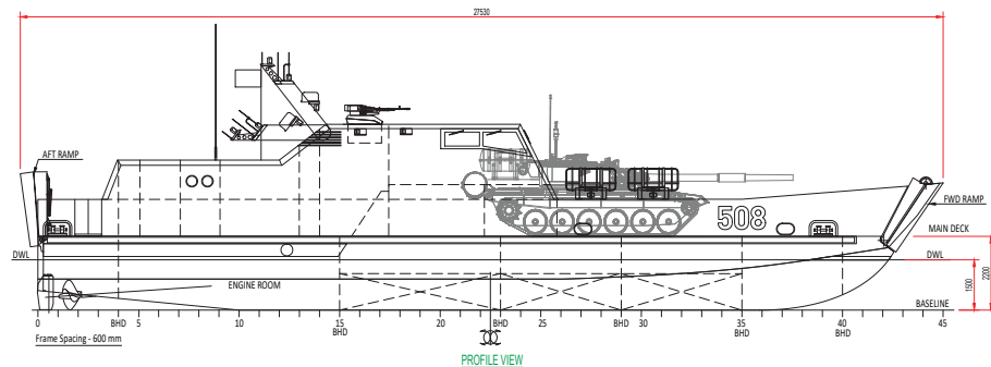
PROFILE VIEW
