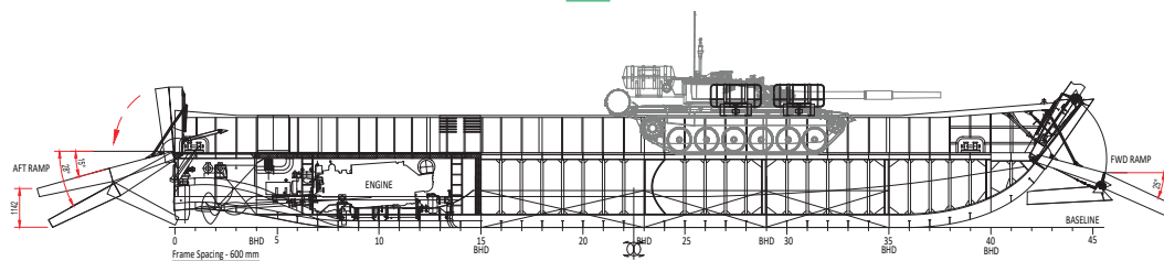
PROFILE VIEW
