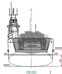
FWD VIEW
