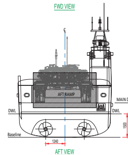
AFT VIEW
